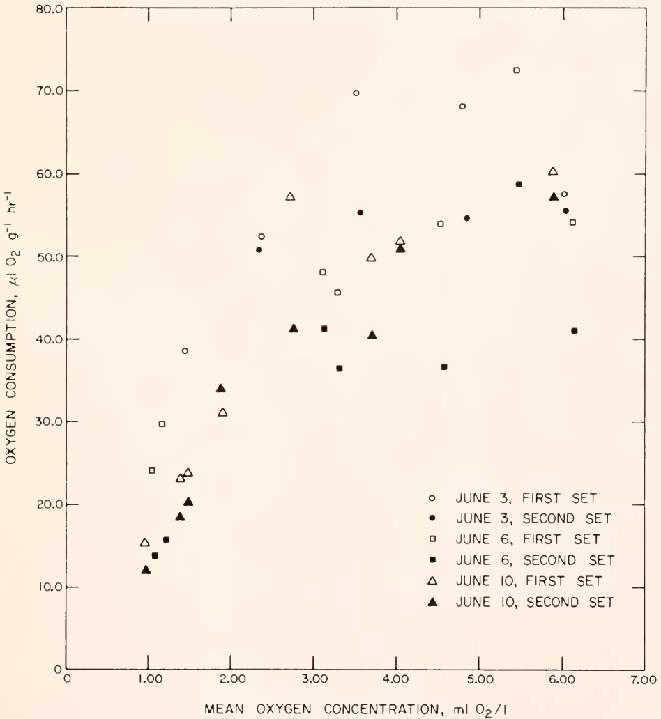
FIGURE 2. Oxygen consumption of Lumbrineris zonata as a function of oxygen concentration.
